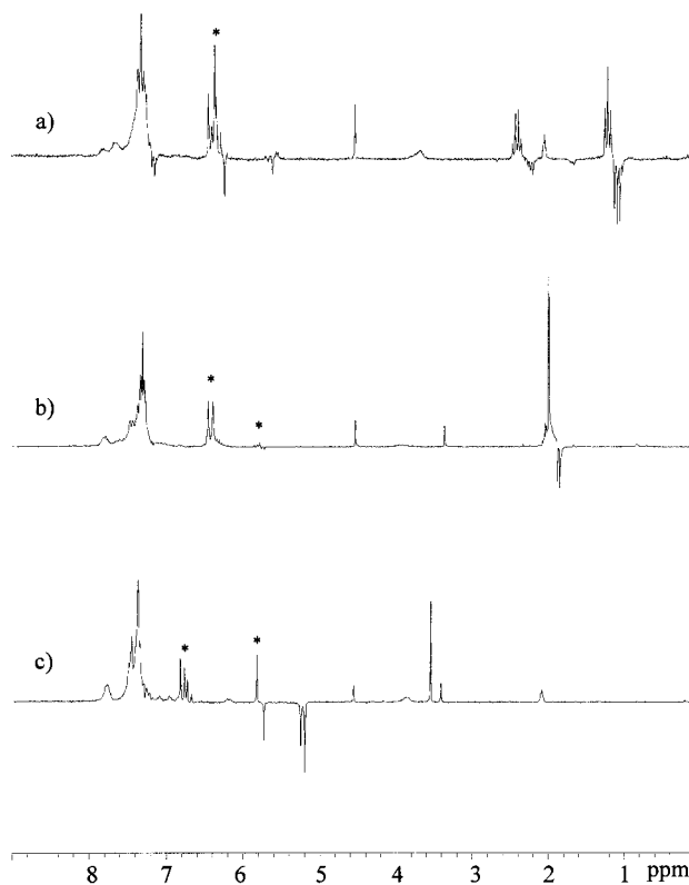
Figure 4. Polarization of product signals during hydrogenation with para- H_2 of alkynes in the presence of [(PPh_3)_2PtHX]/SnX_2 catalytic systems in [D_6] acetone on heating; a ) X = Br, alkyne = 1-phenyl-1-butyne; b ) X = Br, alkyne = 1-phenyl-1-propyne; c ) X = Cl, alkyne = phenylacetylene. The absorption signals of the products, i.e. of the cis -alkenes, are marked *.
