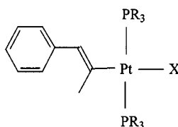
5a X = SnCl 3 5b X = Cl
