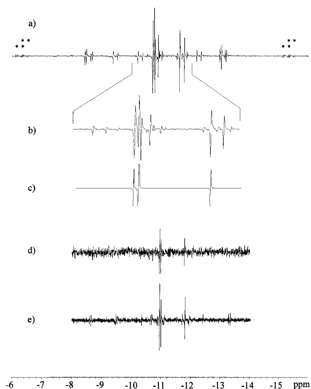
Figure 2. PHIP ^1\text{H} -NMR spectra of the systems \text{trans}[(\text{PPh}_3)_2\text{PtHCl}]/\text{SnCl}_2/\text{alkyne}/\text{para-H}_2 ( [\text{D}_6]\text{acetone} , room temp.): a ) alkyne = 1-phenyl-1-butyne; b ) central lines of the spectrum (a) in the range \delta = -10 to -12 ; c ) PHIP++ simulation of the central part of the spectrum (a); d ) alkyne = diphenylacetylene; e ) alkyne = 3,3-dimethylbutyne
