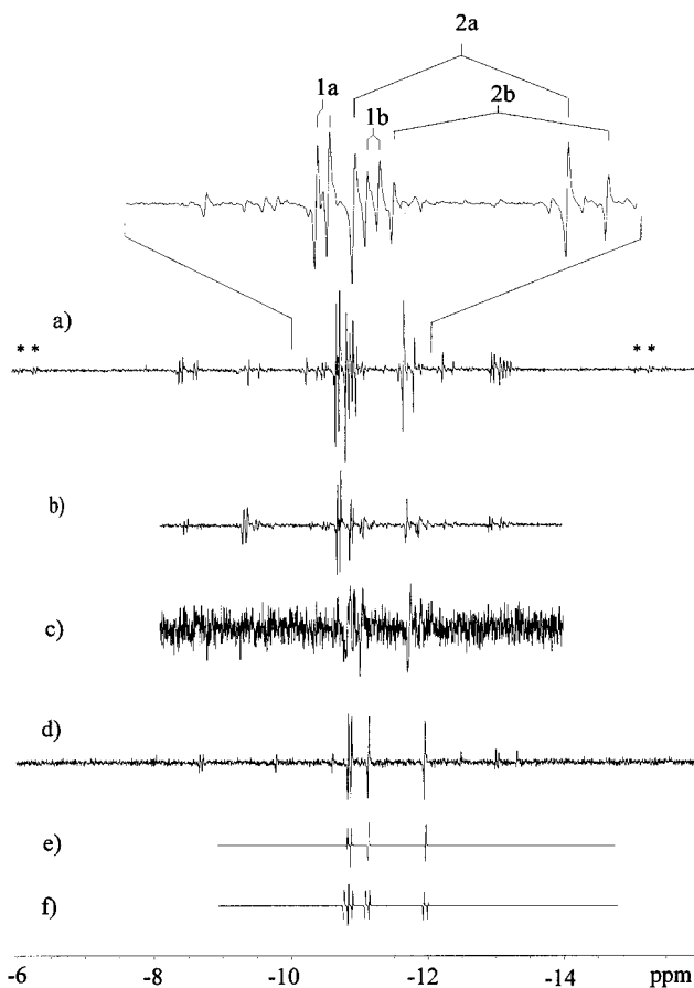
Figure 1. PHIP 1 H-NMR spectra of the system trans -[(PPh 3 ) 2 PtHCl]/SnCl 2 /1-phenyl-1-propyne/para-H 2 in [D 6 ]acetone; a ) at room temp. ( 119 Sn and 117 Sn satellite signals are marked *); b ) the same sample after cooling; c ) PHIP 1 H-NMR spectrum of the isolated insertion product 5a in CD 2 Cl 2 , at 3 bar of para-H 2 , room temp.; d ) PHIP++ simulation of the monophosphane dihydride 6 ; e ) PHIP++ simulation of the diphosphane dihydride 3 (values for cis - and trans -coupling constants are taken to be as in c ); f ) PHIP++ simulation of the diphosphane dihydride 3 (values for cis and trans coupling constants are taken as in c )
