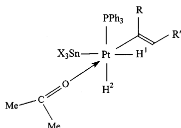
6 a R = Me, R' = Ph, X = Cl; 6 b R = Et, R' = Ph, X = Cl; 6 c R = R' = Ph, X = Cl; 6 d R = H, R' = CMe 3 , X = Cl; 6 e R = R' = Ph, X = Br
