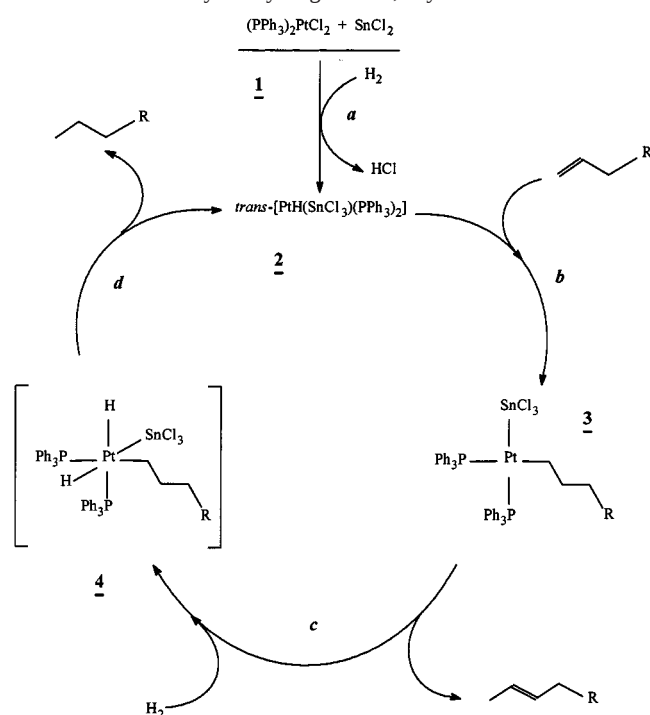
Scheme 1. Generally assumed mechanism for the Pt II –tin dichloride catalyzed hydrogenation, asynchronous mechanism
