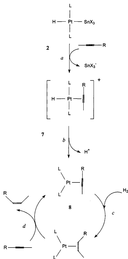
Scheme 2. The proposed mechanism for the synchronous hydrogenation of alkynes catalyzed with the [(PR 3 ) 2 PtHX]–SnX 2 system in acetone
