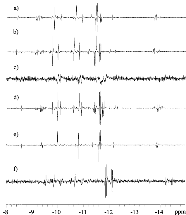
Figure 3. PHIP ^1\text{H} -NMR spectra of the systems [\text{L}_2\text{PtHBr}]/\text{SnBr}_2/\text{alkyne}/\text{para-H}_2 in [\text{D}_6]\text{acetone} : a ) \text{L} = \text{PPh}_3 , alkyne = 1-phenyl-1-propyne, room temp.; b ) \text{L} = \text{PPh}_3 , alkyne = 1-phenyl-1-butyne, room temp., before heating; c ) \text{L} = \text{PPh}_3 , alkyne = 1-phenyl-1-butyne, on heating; d ) \text{L} = \text{PPh}_3 , alkyne = 1-phenyl-1-butyne, at room temp. after heating; e ) \text{L} = \text{PPh}_3 , alkyne = diphenylacetylene, room temp.; f ) \text{L} = \text{PMePh}_2 , alkyne = 1-phenyl-1-propyne, room temp.
